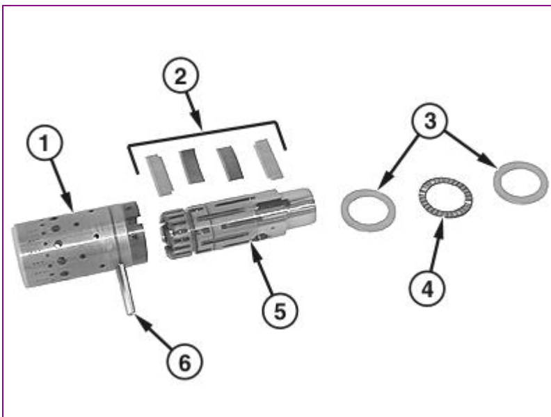
2. T217479A-UN: Exploded View of Spool Valve Assembly
