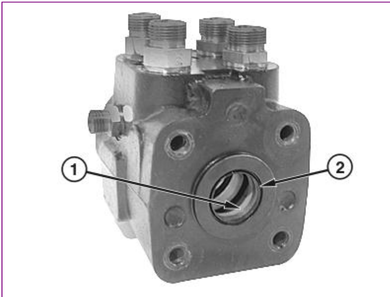
1. T217478A-UN: Steering Valve Seals
